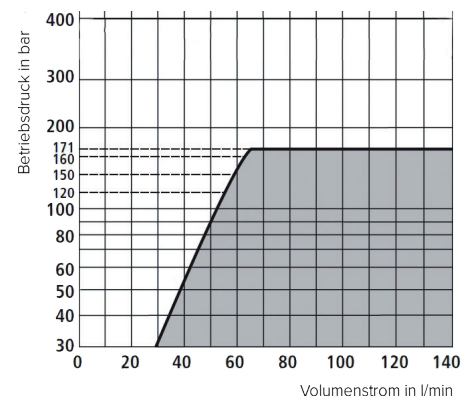
Volume flows via pressure discharge valve P to T, volume flows in the grey area cannot be displayed
